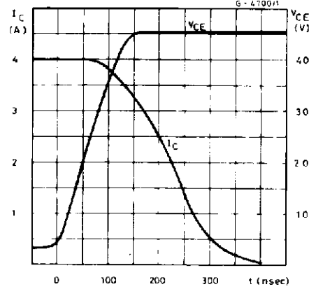
Figure 6. Turn-off Phase.
